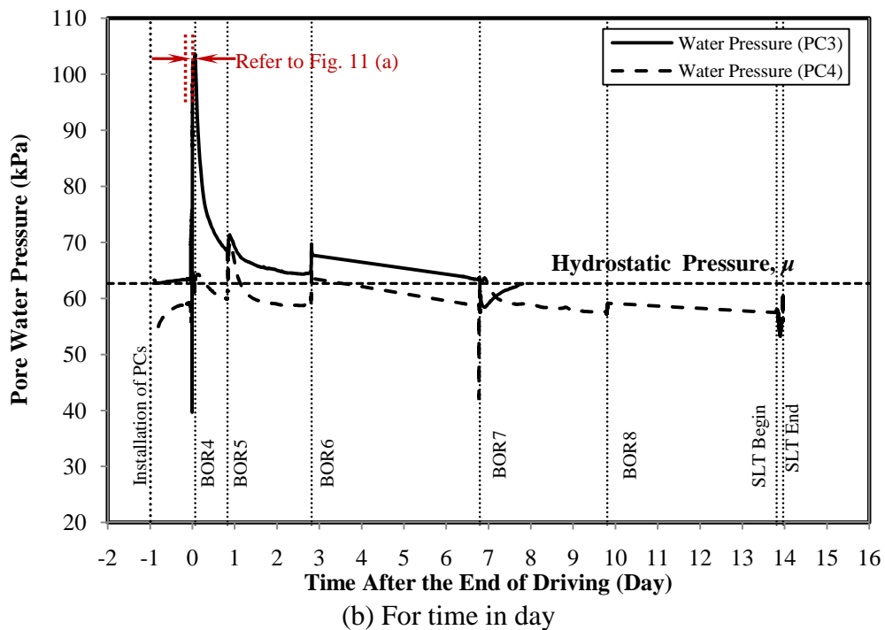
Figure 3.13: Pore water pressure recorded by push-in pressure cells (PC3 and PC4) at ISU6 as function of time considered after EOD in (a) minutes; and (b) days
