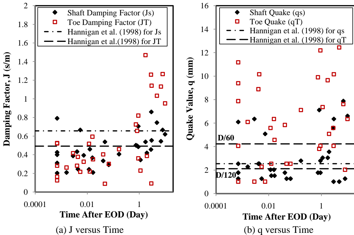
Figure 7.5: Time measured after EOD versus (a) damping factors; and (b) quake values obtained from recently completed field tests using CAPWAP for cohesive soils
