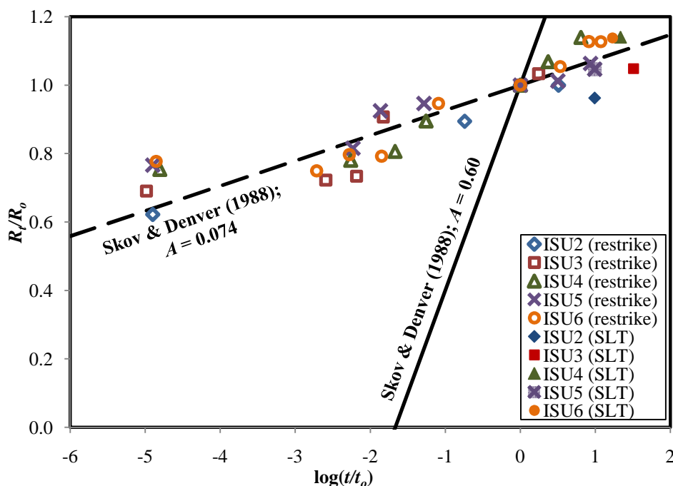
Figure 4.1: Comparison between ISU field test results and Skov and Denver (1988) pile setup method
