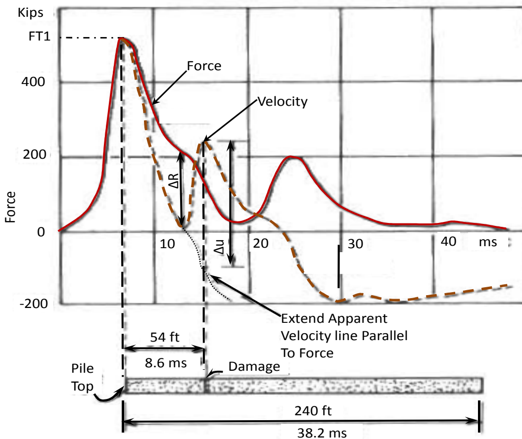
Figure 2.4: A typical pile damage force and velocity record (after Rausche and Goble, 1979)
