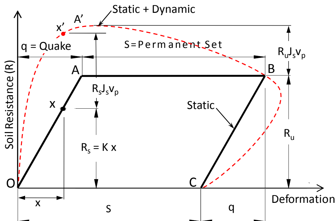
Figure 2.7: Stress strain diagram of the soil resistance at a pile point (after Coyle and Gibson, 1970 and Smith, 1962).
