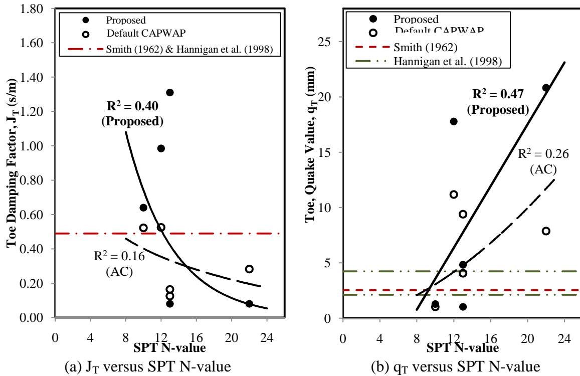
Figure 7.23: SPT N-value versus (a) toe damping factor; and (b) toe quake value for cohesive soils
