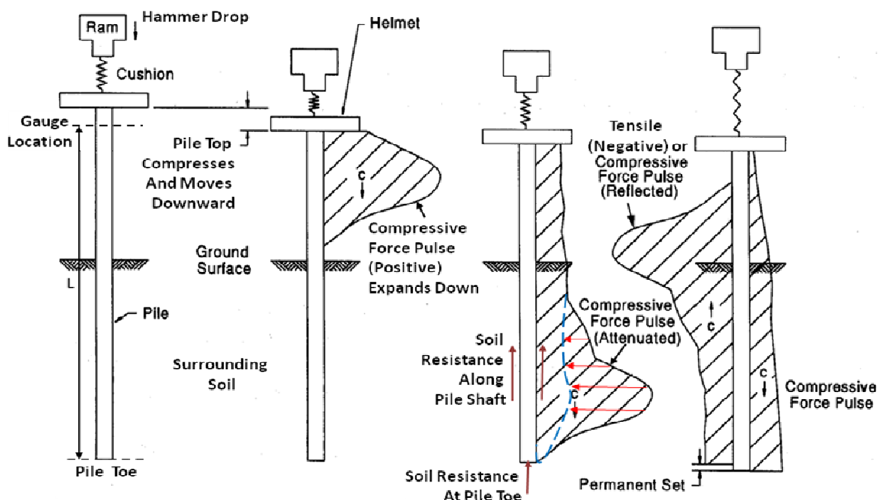
Figure 2.3: Wave propagation in a pile (adapted and modified from Cheney and Chassie, 1993)
