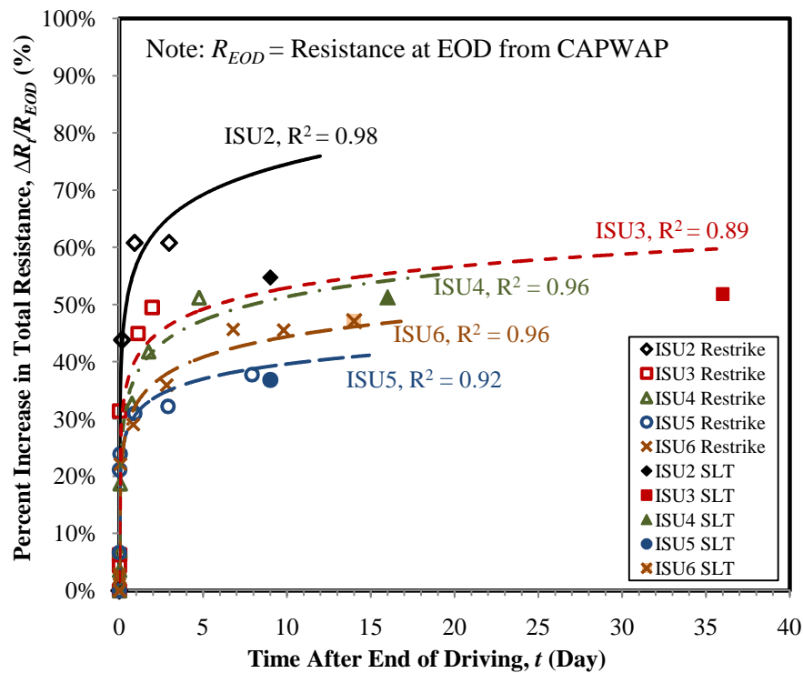
Figure 3.12: Percent increase in total resistance for all five test piles
